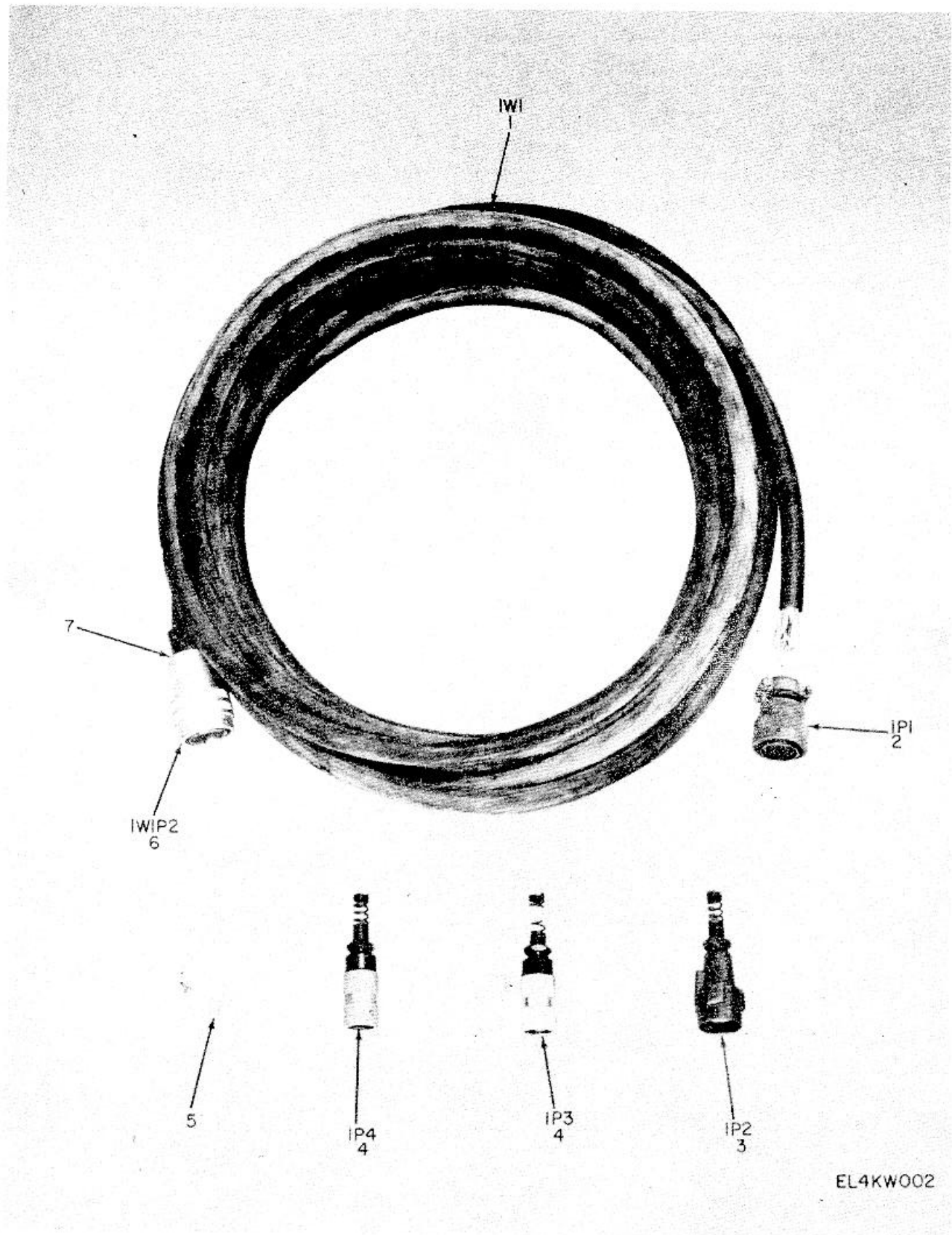
Figure 2. Cable Assembly Kit.
